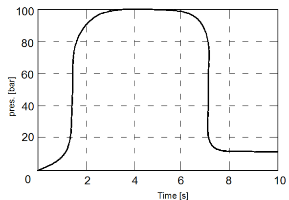
Fig. 7. Pressure diagram
