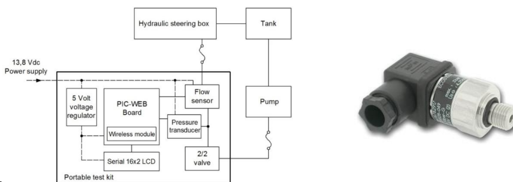
Fig. 2. Block diagram and the transducer circuit of portable test equipment with data transmission
