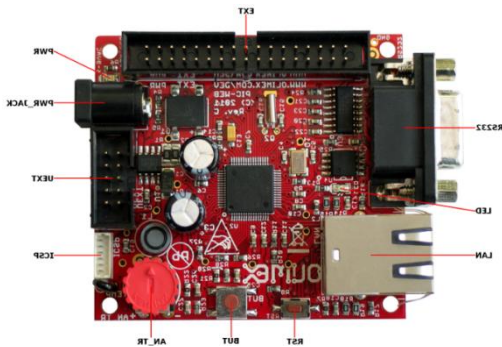
Fig. 3. The Pic-Web electronic development board from Olimex
