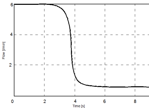
Fig. 6. Flow diagram
