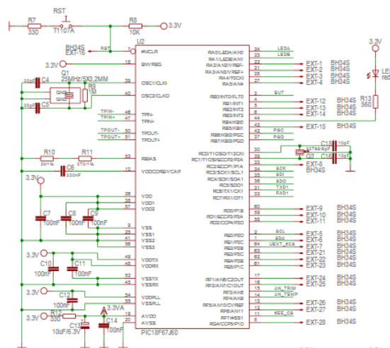
Fig. 4. The electronic diagram of the electronic module with microcontroller
